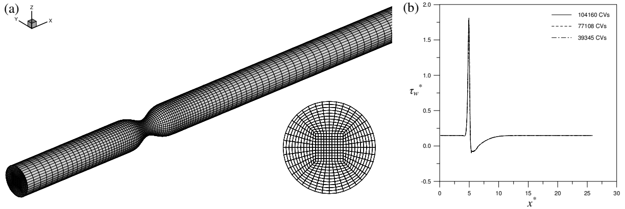
Figure 2: (a) 3D grid with cross-section; (b) Grid refinement study by comparison of the dimensionless wall shear stress for three grid resolutions
