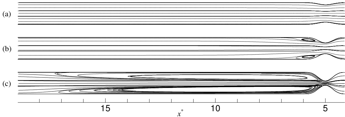
Figure 6: Streamlines for Casson- based flow at Re=100 and for different degrees of stenosis: (a) 20%; (b) 50%; (c) 80%.
